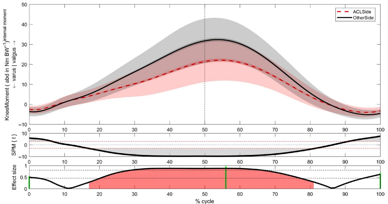
FIGURE 4 Differences in knee valgus moment between limbs during hurdle hop. The top panel illustrates the mean and SD clouds for the ACLR and non-ACLR limbs. The middle panel illustrates the SPM{t} – the t-statistic as a function of time describing the difference between the two limbs. The red line represents the critical threshold and the shaded portion of the curve indicates p < 0.05 – a significant difference between the limbs. The bottom panel illustrates the effect size as a function of time describing the magnitude of the effect. In the bottom panel the dotted lines represent the thresholds for Cohen's d > 0.5 and d > 0.8 . The shaded portion indicates that the average Cohen's d > 0.5 with red indicating a large effect size across that phase.
