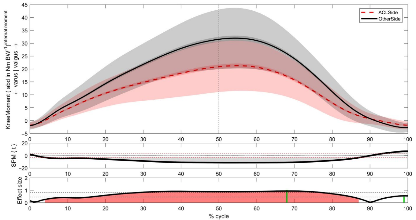
FIGURE 1 Knee valgus moment between limbs during double leg drop jump. The top panel illustrates the mean and SD clouds for the ACLR (red dash) and non-ACLR limbs (black solid). The middle panel illustrates the SPM{t} – the t-statistic as a function of time describing the difference between the two limbs. The red line represents the critical threshold and the shaded portion of the curve indicates p < 0.05 - a significant difference between the limbs. The bottom panel illustrates the effect size as a function of time describing the magnitude of the effect. The dotted lines represent the thresholds for Cohen’s d > 0.5 and d > 0.8 . The shaded portion indicates that the average Cohen’s d > 0.5 with red indicating a large effect size across that phase.
