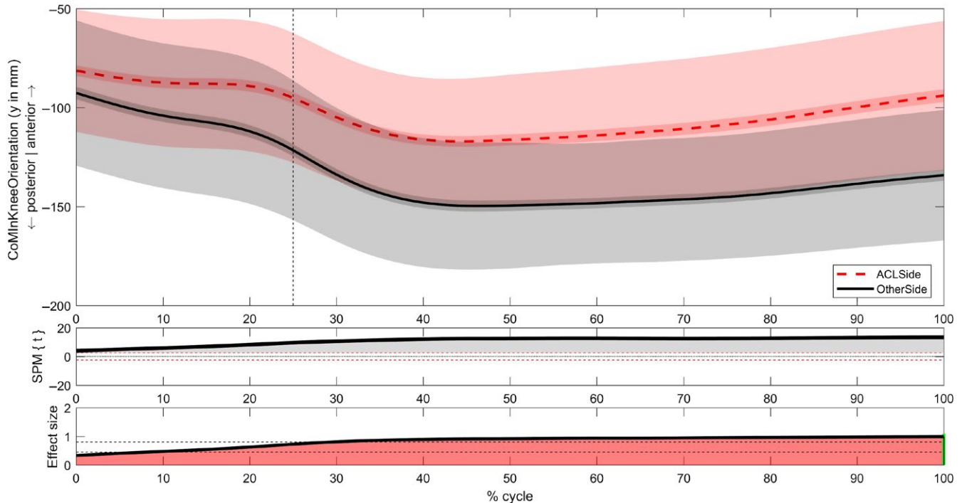
FIGURE 3 Difference in position of COM posterior to knee between limbs during single leg hop for distance. Top panel illustrates the mean and SD clouds for the ACLR and non-ACLR limbs. The middle panel illustrates the SPM{t} – the t-statistic as a function of time describing the difference between the two limbs. The red line represents the critical threshold and the shaded portion of the curve indicates p < 0.05 – a significant difference between the limbs. The bottom panel illustrates the effect size as a function of time describing the magnitude of the effect. The dotted lines represent the thresholds for Cohen's d > 0.5 and d > 0.8 . The shaded portion indicates that the average Cohen's d > 0.5 with red indicating a large effect size across that phase.
