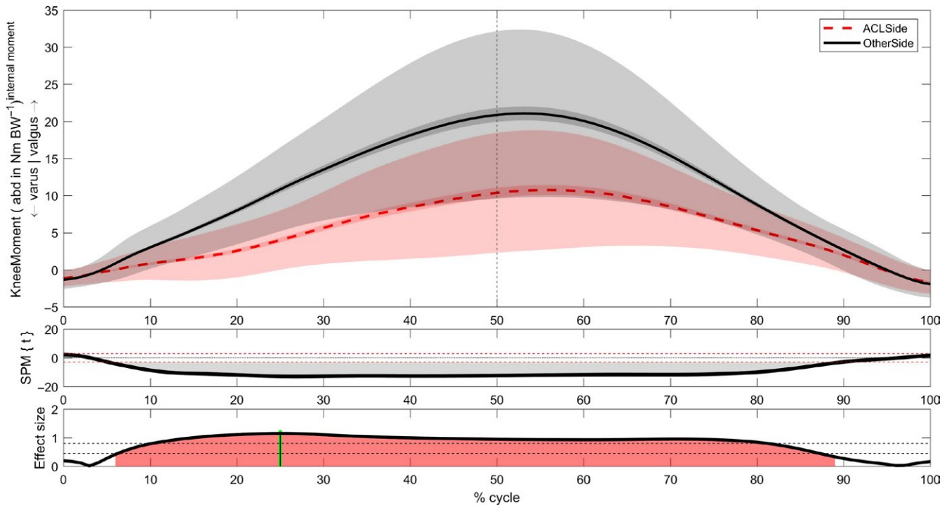
FIGURE 2 Difference in knee valgus moment between limbs during single leg drop jump. The top panel illustrates the mean and SD clouds for the ACLR and non-ACLR limbs. The middle panel illustrates the SPM\{t\} – the t-statistic as a function of time describing the difference between the two limbs. The red line represents the critical threshold and the shaded portion of the curve indicates p < 0.05 – a significant difference between the limbs. In the bottom panel the dotted lines represent the thresholds for Cohen's d > 0.5 and d > 0.8 . The shaded portion indicates that the average Cohen's d > 0.5 with red indicating a large effect size across that phase.
